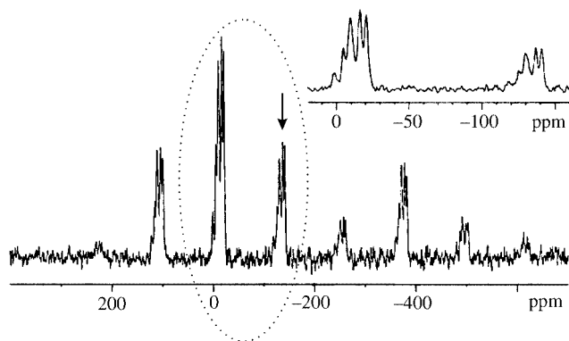
Figure 3. 119 Sn CP/MAS NMR spectrum of bis(3-methoxypropyl)tin dichloride ( 3 ); the vertical arrow indicates the centre band
