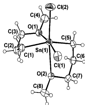
Figure 1. Solid-state structure of bis(3-methoxypropyl)tin dichloride ( 3 )
