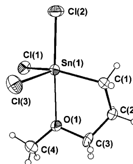
Figure 2. Solid-state structure of (3-methoxypropyl)tin trichloride ( 4 )
